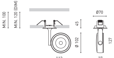
SIX L RECESSED
