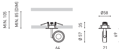
SIX S RECESSED
