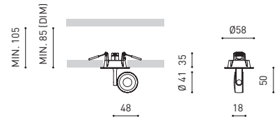
SIX XS RECESSED
