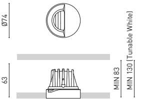
BUDDY WALL WASHER TRIMLESS
