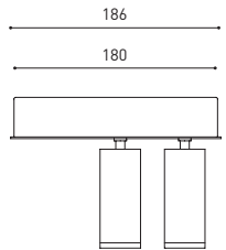
FIT 35 SURFACE DOUBLE
