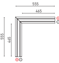
BRIGHT LINE CORNER 90° ONE PLANE POLARIZED A
