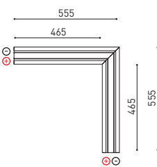
BRIGHT LINE CORNER 90° ONE PLANE POLARIZED B
