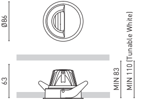
BUDDY WALL WASHER
