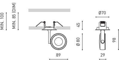
SIX M RECESSED
