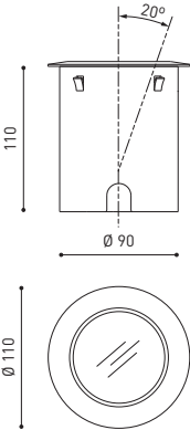
DARK M ASYMMETRIC
